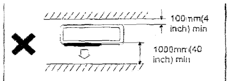
3. When there are obstacles only in the front (air outlet)
